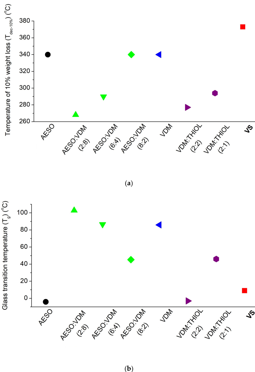
Figure 5. Comparison of the temperature of the 10% weight loss (a) and the glass transition temperature (b) of the polymer VS and the polymers of AESO [33], VDM [35], AESO and VDM [34], VDM and THIOL [15]. The molar ratio of the monomers is presented in parentheses.
