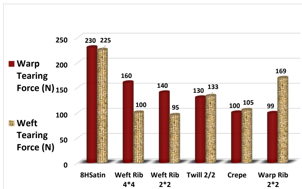
Figure 1. Effect of fabric structure on the tearing force in the warp and weft directions. Reproduced with permission from [48]. Copyright 2018 Elsevier.
