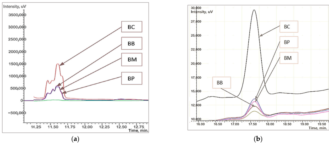
Figure 7. Peak area of HPLC chromatogram of wheat bran samples gliadin extract after incubation of 4 h at 45 °C: (a) \omega -gliadins; (b) \alpha -gliadins (BC, control bran sample; BB, bran treated with bromelain; BP, bran treated with papain; BM, bran treated with a combination of bromelain and papain).
