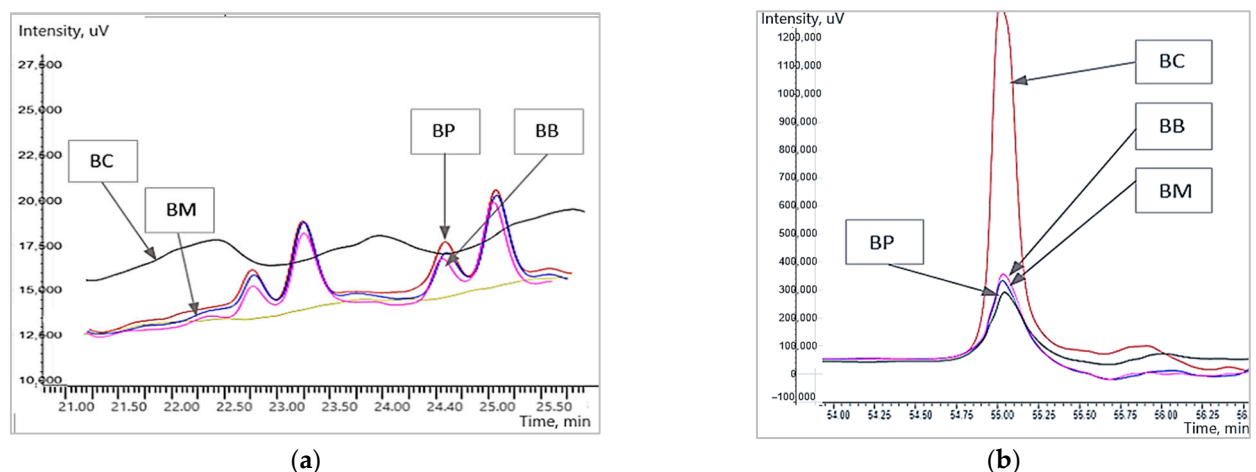
Figure 8. Peak area of HPLC chromatogram of wheat bran samples gliadin extract after incubation: (a) gliadin degradation products; (b) \gamma -gliadins (BC, control bran sample; BB, bran treated with bromelain; BP, bran treated with papain; BM, bran treated with a combination of bromelain and papain).
