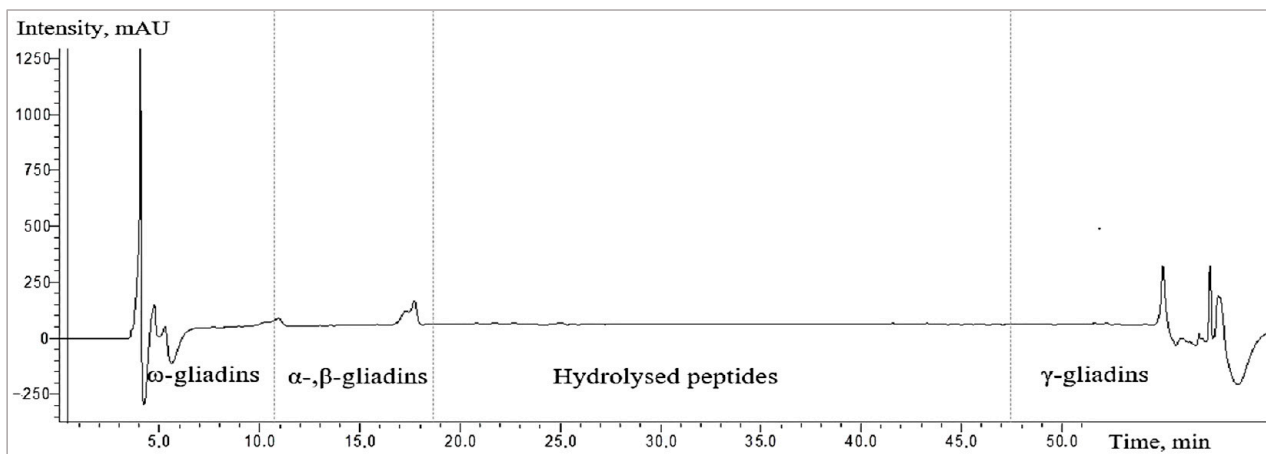
Figure 6. HPLC chromatogram of gliadin fraction of wheat bran samples treated with bromelain 4 h at 45 °C.
