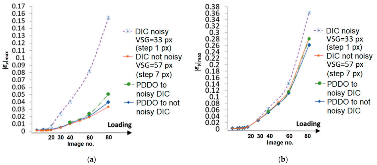
Figure 14. Effect of the input noise on the calculated strains at different levels of deformation: (a) \epsilon_x strains, (b) \epsilon_y strains.
