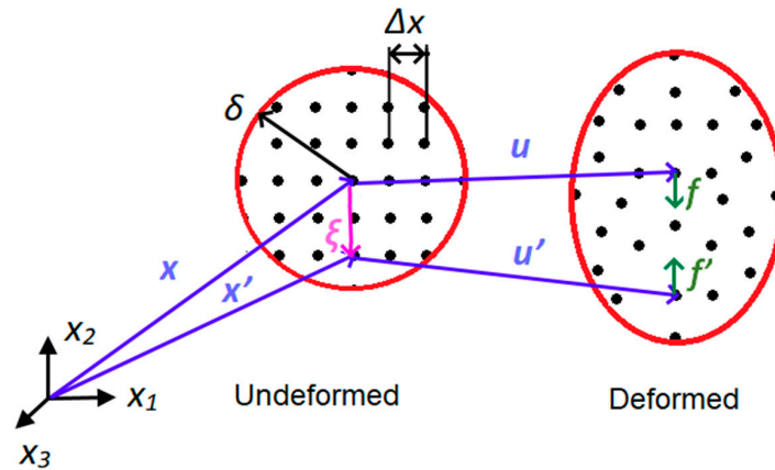
Figure 4. The basic principles of the PD theory.
