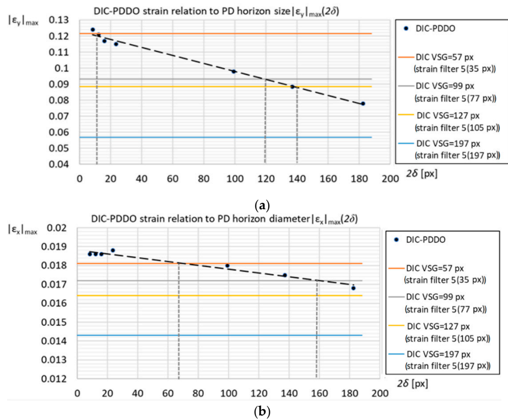
Figure 8. Effect of the PD horizon size on the strain values computed on in-house tensile experiment specimen surface by the DIC-PDDO method: (a) \epsilon_y strains, (b) \epsilon_x strains.
