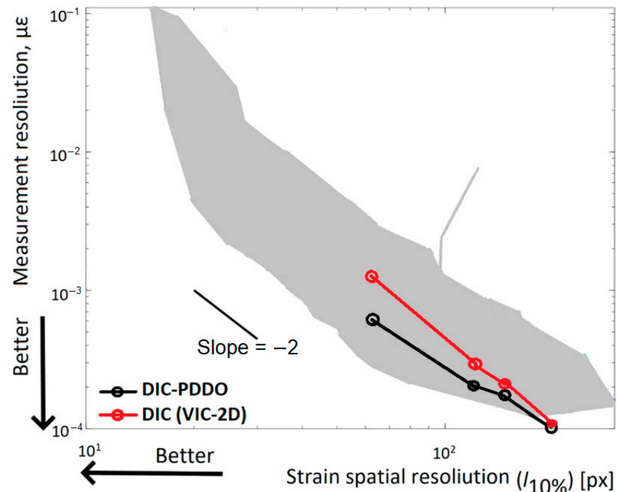
Figure 11. Comparison of the DIC strain calculation algorithms (the data points replicated from [35] are marked as grey area) and DIC-PDDO method.
