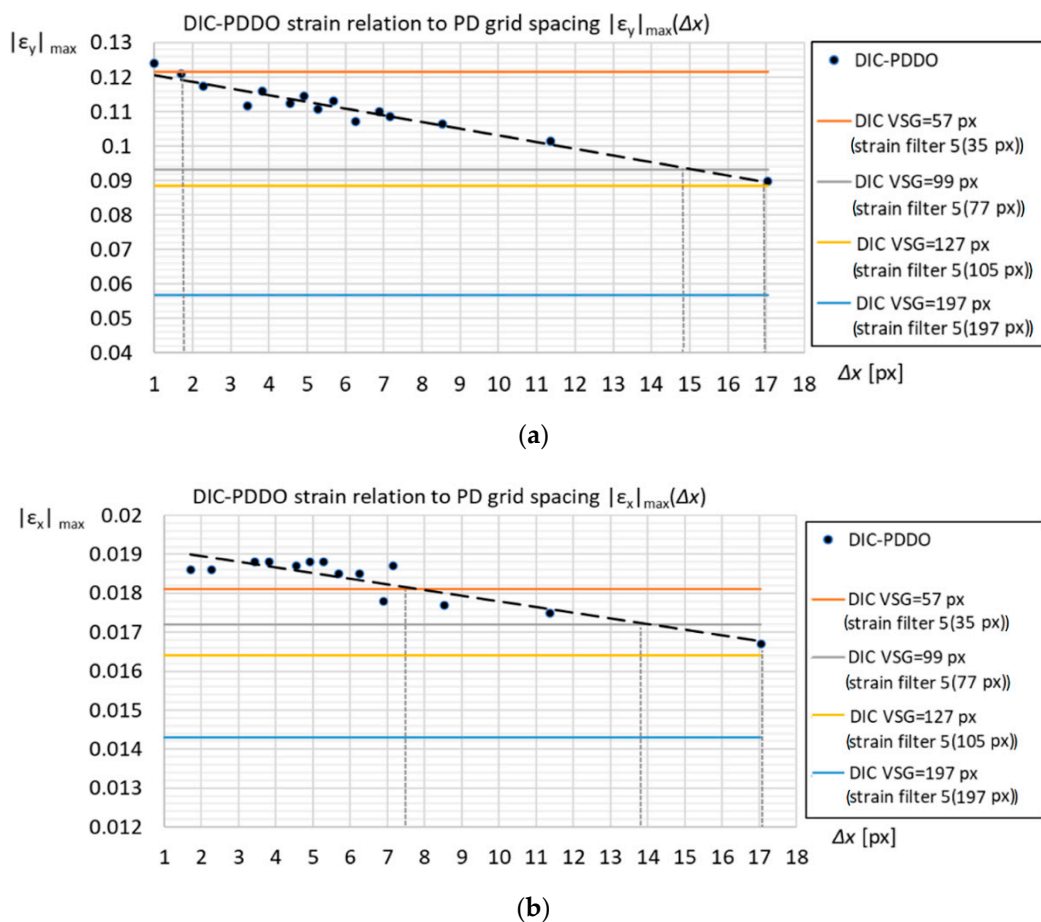
Figure 7. Effect of the PD grid spacing \Delta x on the strain values computed on in-house tensile experiment specimen surface by the DIC-PDDO method ( \delta = 3.1\Delta x ): (a) \varepsilon_y strains, (b) \varepsilon_x strains.
