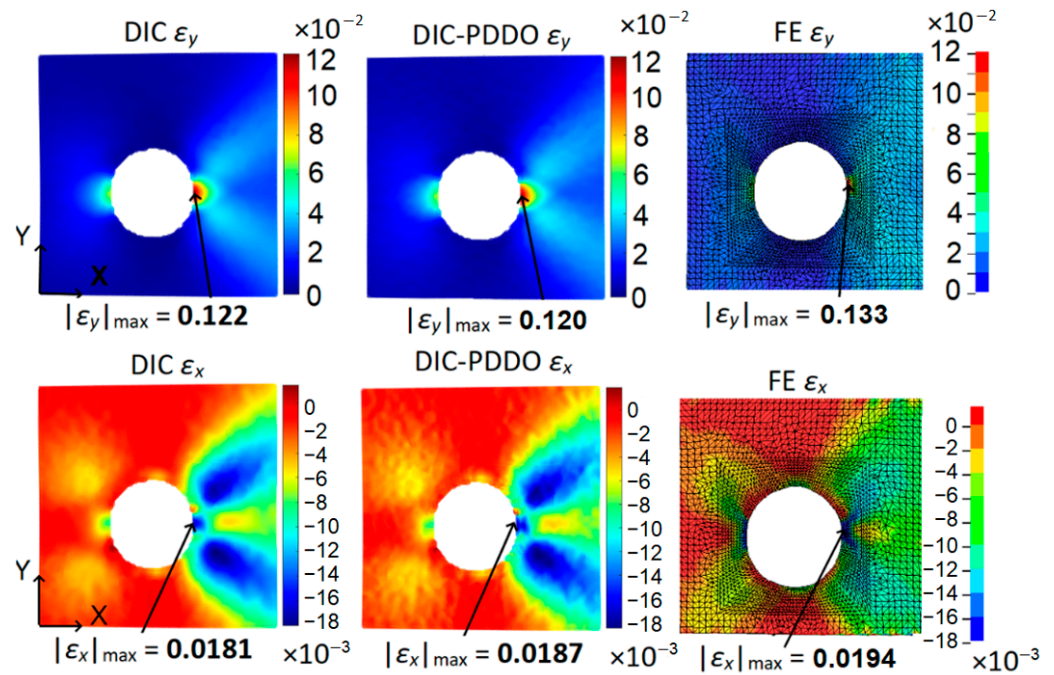
Figure 9. Comparison of \epsilon_y, \epsilon_x Lagrangian strains computed on tensile experiment specimen with DIC (VSG = 57 px), DIC-PDDO ( \delta = 3.1\Delta x, \Delta x = 0.167 mm) and FE simulation.
