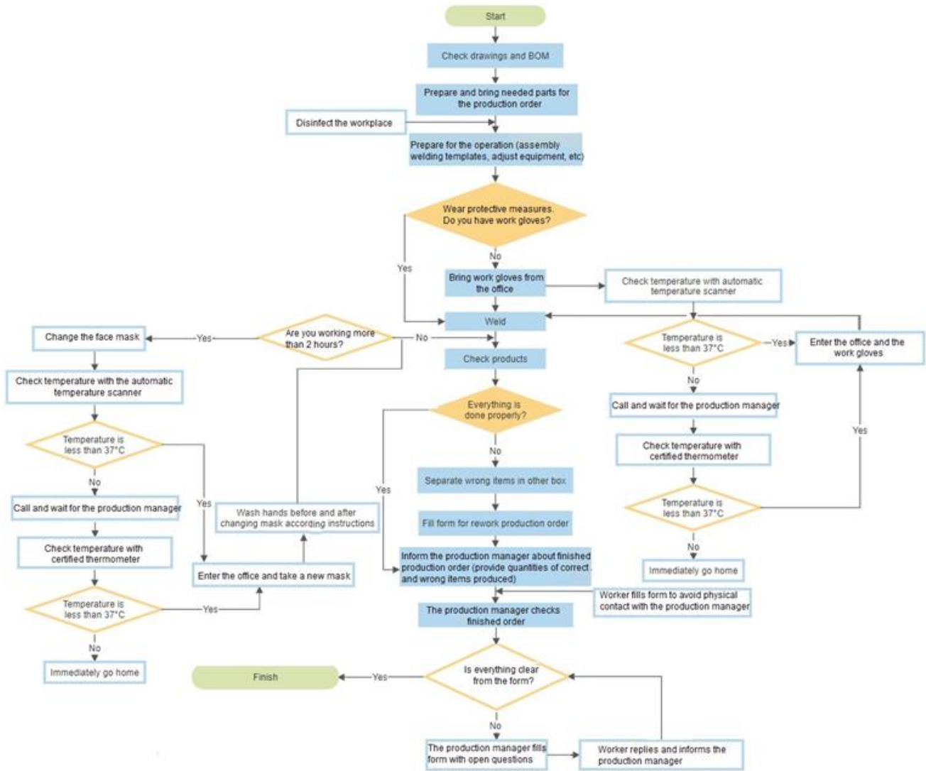
Fig. 2 Algorithm of welding operation
