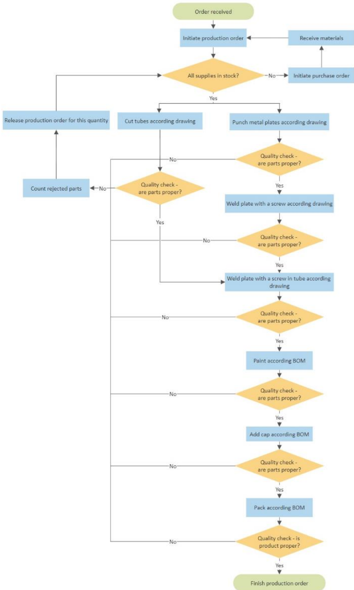
Fig. 1 Workflow of metal leg production
