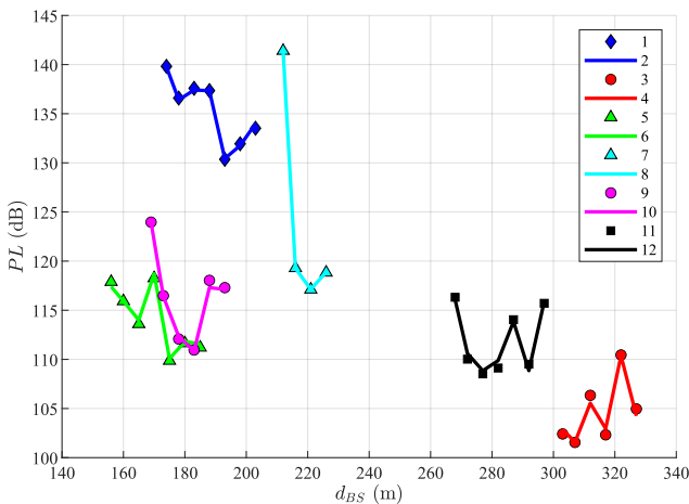
Fig. 8: Comparison of Model, see Eq. (13), and the experimental results for the UMTS technology: 6 m experiment - 1, 14 m experiment - 3, 18/1 m experiment - 5, 18/2 m experiment - 7, 23 m experiment - 9, 32 m experiment - 11, 6 m model - 2, 14 m model - 4, 18/1 m model - 6, 18/2 m model - 8, 23 m model - 10, 32 m model - 12.
