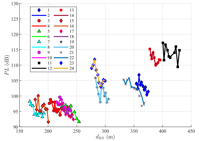
Fig. 9: Comparison of Model, see Eq. (13), and the experimental results for the GSM technology: 12/1 m experiment - 1, 12/2 m experiment - 3, 15/1 m experiment - 5, 15/2 m experiment - 7, 15/3 m experiment - 9, 18/3 m experiment - 11, 18/4 m experiment - 13, 18/5 m experiment - 15, 22 m experiment - 17, 35/1 m experiment - 19, 35/2 m experiment - 21, 41 m experiment - 23, 12/1 m model - 2, 12/2 m model - 4, 15/1 m model - 6, 15/2 m model - 8, 15/3 m model - 10, 18/3 m model - 12, 18/4 m model - 14, 18/5 m model - 16, 22 m model - 18, 35/1 m model - 20, 35/2 m model - 22, 41 m model - 24.
