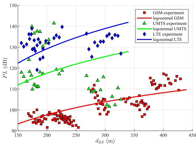
Fig. 3: Data comparison of path losses with the log-normal path losses model for the different mobile technologies.
