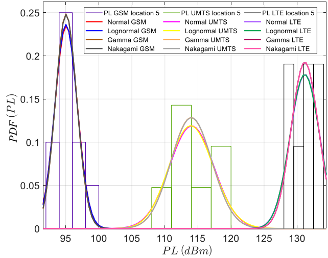
Fig. 5: Comparison of the experimental path losses PDF fitting.
