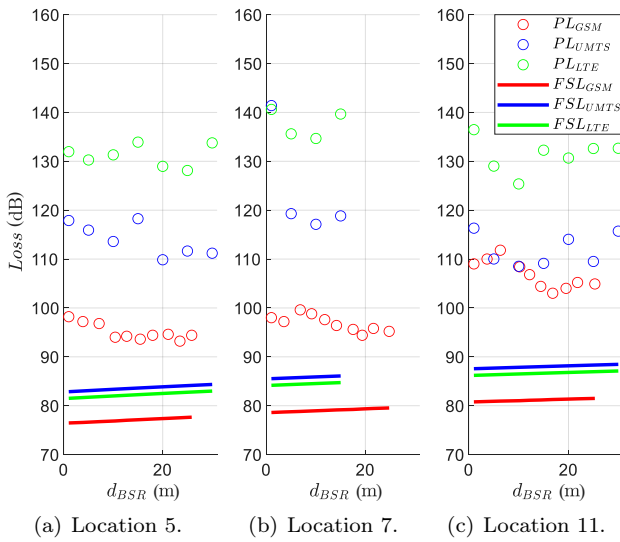
Fig. 4: Experimental path and theoretical free space losses as a function of the distance d_{BSR} .
