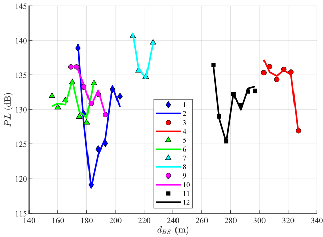
Fig. 7: Comparison of Model, see Eq. (13), and the experimental results for the LTE technology: 6 m experiment - 1, 14 m experiment - 3, 18/1 m experiment - 5, 18/2 m experiment - 7, 23 m experiment - 9, 32 m experiment - 11, 6 m model - 2, 14 m model - 4, 18/1 m model - 6, 18/2 m model - 8, 23 m model - 10, 32 m model - 12.
