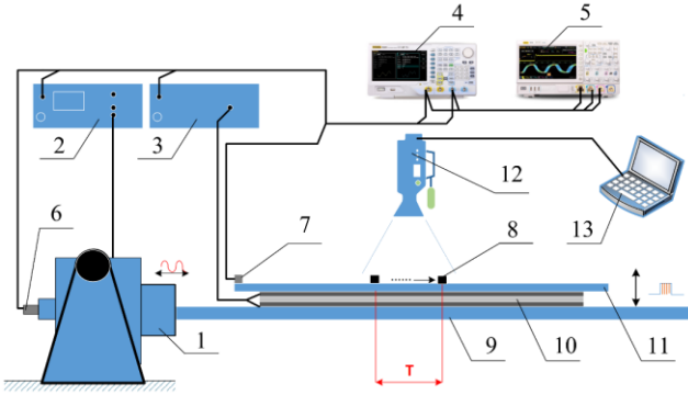
Fig. 5 Scheme of experimental setup: 1 – electrodynamic shaker; 2 – low-frequency vibration amplifier; 3 – high-frequency vibration amplifier; 4 – arbitrary waveform generator; 5 – digital oscilloscope; 6, 7 – vibration sensors; 8 – micropart; 9 – platform base subjected to sinusoidal displacement cycles; 10 – piezoelectric actuator; 11 – platform for conveying; 12 – camera; 13 – computer
