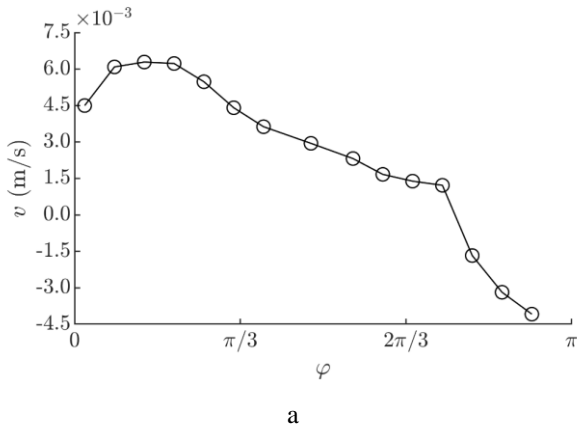
Fig. 9 Experimental average stable conveying velocity v depending on: a) the phase shift \varphi , A = 0.16 mm, \omega = 125.7 rad/s, \Delta\tau = 7\pi/15 ; b) \Delta\tau , A = 0.16 mm, \varphi = \pi/2
