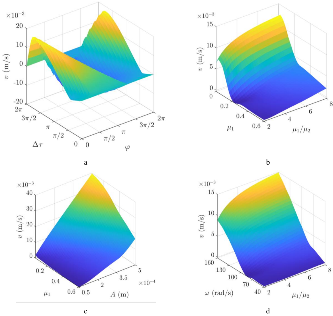
Fig. 4 Three-dimensional representation of the average stable conveying velocity as a function of: a) the phase shift and \Delta\tau ; b) the nominal dry friction coefficient and the ratio of friction reduction; c) the nominal dry friction coefficient and the amplitude of sinusoidal displacement cycles; d) the angular frequency of sinusoidal displacement cycles and the ratio of friction reduction
