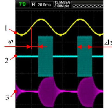
Fig. 7 Oscillograms of the system's signals: 1 – signal for sinusoidal displacement cycles; 2 – signal of high frequency pulses in burst mode for dry friction control; 3 – vibrational response of the platform
