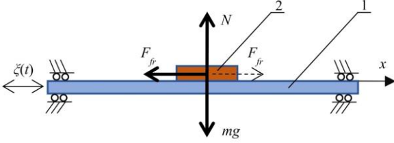
Fig. 1 The dynamic model of part conveying with dry friction control in respect of sinusoidal displacement cycles: 1 – platform with a possibility to control dry friction; 2 – part for conveyance
