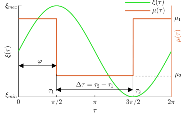
Fig. 2 Dry friction control in respect of the sinusoidal displacement period
