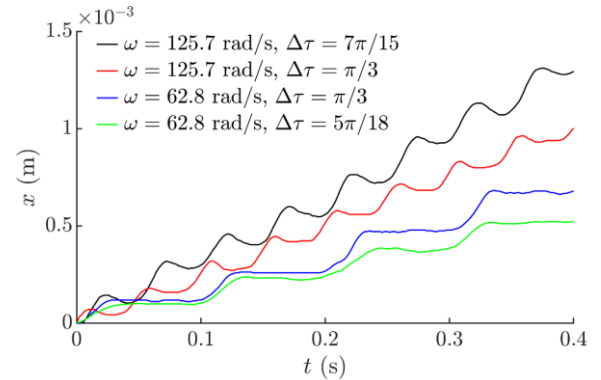
Fig. 8 Captured displacement of micropart over time at different \omega and \Delta\tau values, A = 0.16 mm, \varphi = \pi/2
