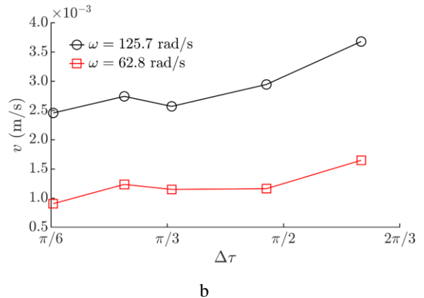
Fig. 9 Experimental average stable conveying velocity v depending on: a) the phase shift \varphi , A = 0.16 mm, \omega = 125.7 rad/s, \Delta\tau = 7\pi/15 ; b) \Delta\tau , A = 0.16 mm, \varphi = \pi/2
