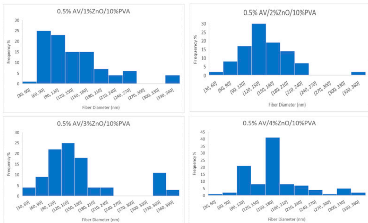
Figure 6. Diameter Distribution of electrospun nanofiber samples 5, 6, 7 and 8 containing 1%, 2%, 3% and 4% ZnO NPs, respectively, with constant amounts of aloe vera and PVA.
