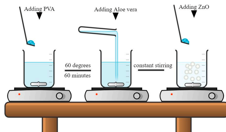
Figure 1. Aloe vera/PVA/ZnO solution formation process for electrospinning.
