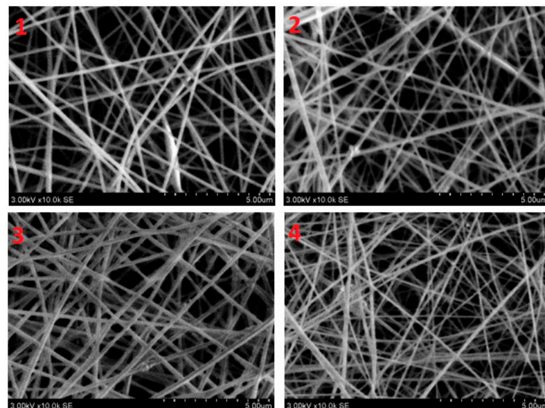
Figure 3. SEM images of electrospun nanofibers: “1”—10% PVA/1% aloe vera/0.5% ZnO NPS; “2”—10% PVA/2% aloe vera/0.5% ZnO NPS; “3”—10% PVA/3% aloe vera/0.5% ZnO NPS; and “4”—10% PVA/4% aloe vera/0.5% ZnO NPS.
