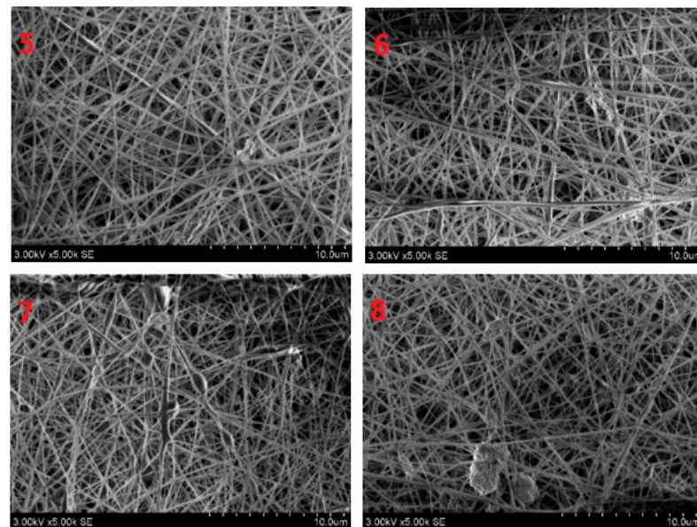
Figure 5. SEM Images of electrospun nanofibers: “5”—10% PVA/0.5% aloe vera/1% ZnO NPs; “6”—10% PVA/0.5% aloe vera/2% ZnO NPs; “7”—10% PVA/0.5% aloe vera/3% ZnO NPs; “8”—10% PVA/0.5% aloe vera/4% ZnO NPs.
