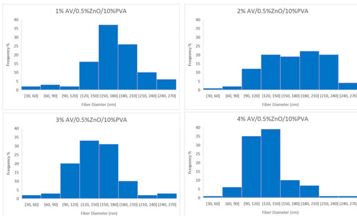
Figure 4. Diameter distribution of developed nanofibers in samples 1, 2, 3 and 4 with 1%, 2%, 3% and 4% aloe vera, respectively, and containing constant amount of ZnO and PVA.
