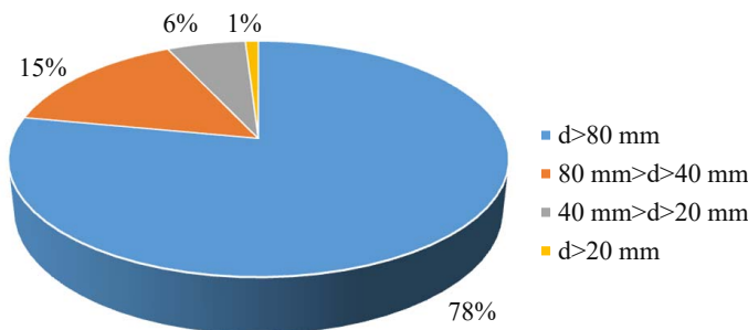
Fig. 1. Granulometric composition of the obtained RDF
