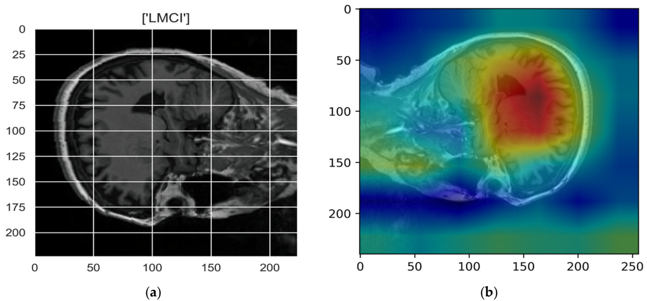
Figure 14. Grad-CAM explanation for the prediction of class LMCI: (a) MRI image, (b) Grad-CAM attention map.
