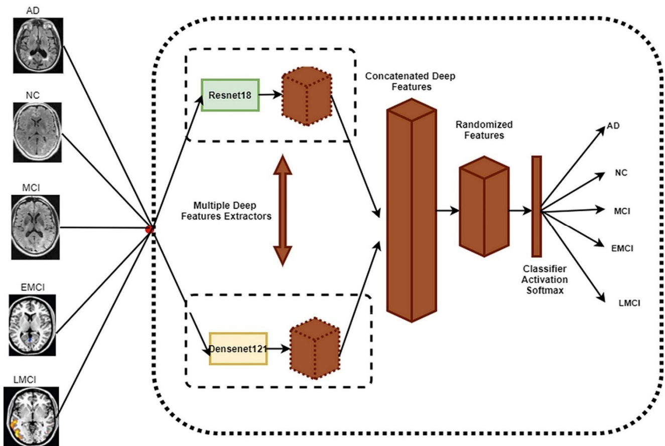
Figure 1. The main framework for the proposed method.
