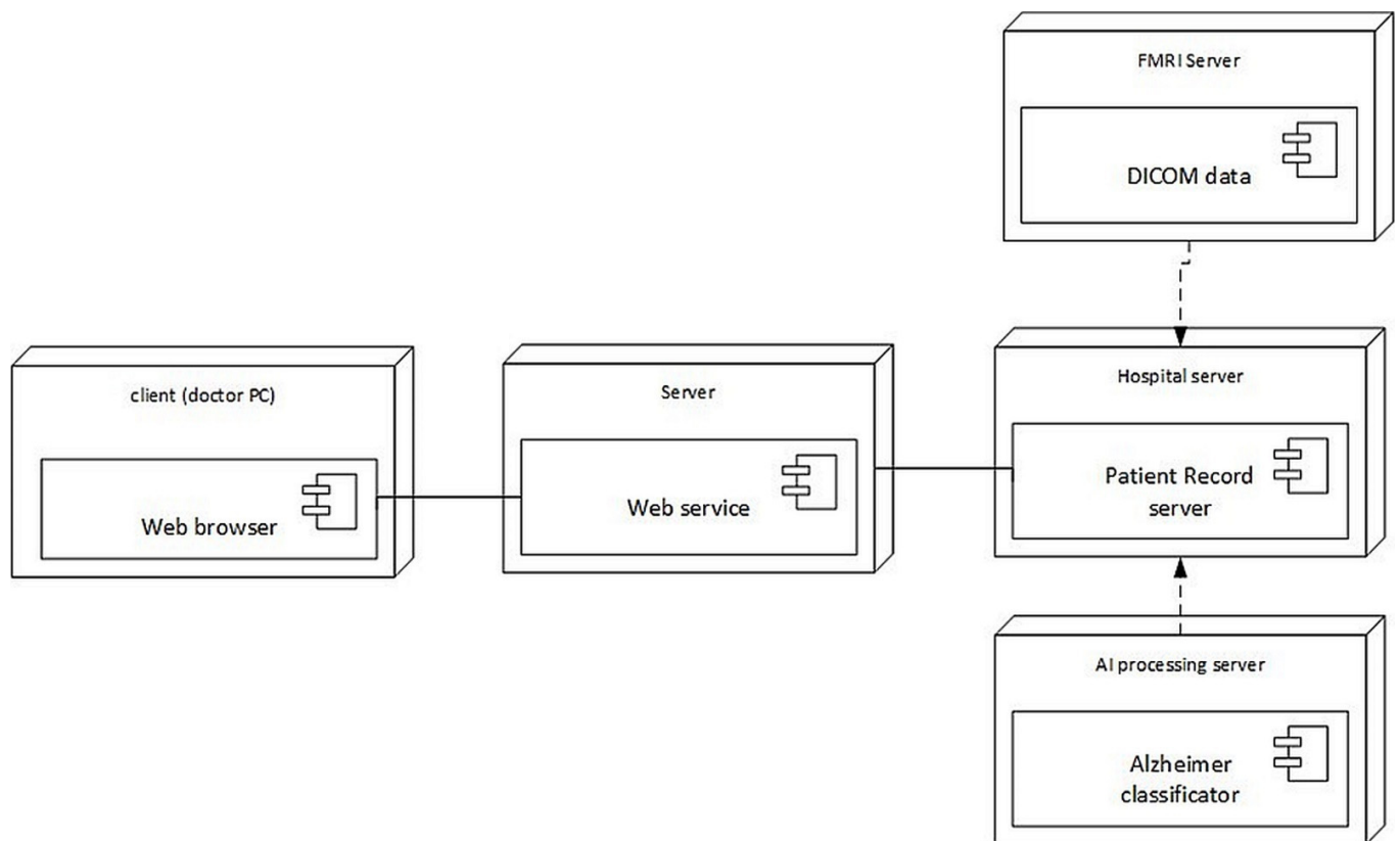
Figure 5. Deployment of the developed system architecture.
