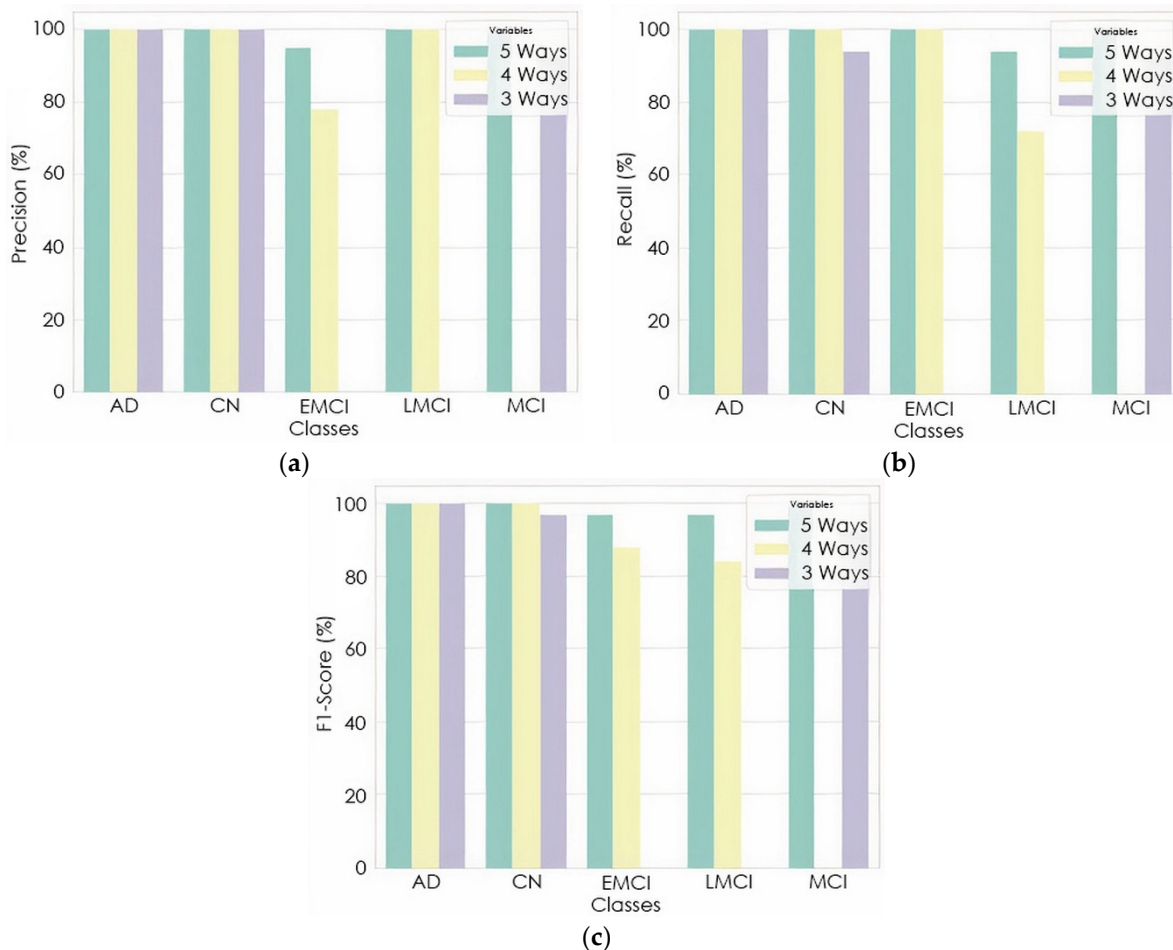
Figure 8. Per class classification report: (a) precision; (b) recall; (c) F1-Score.
