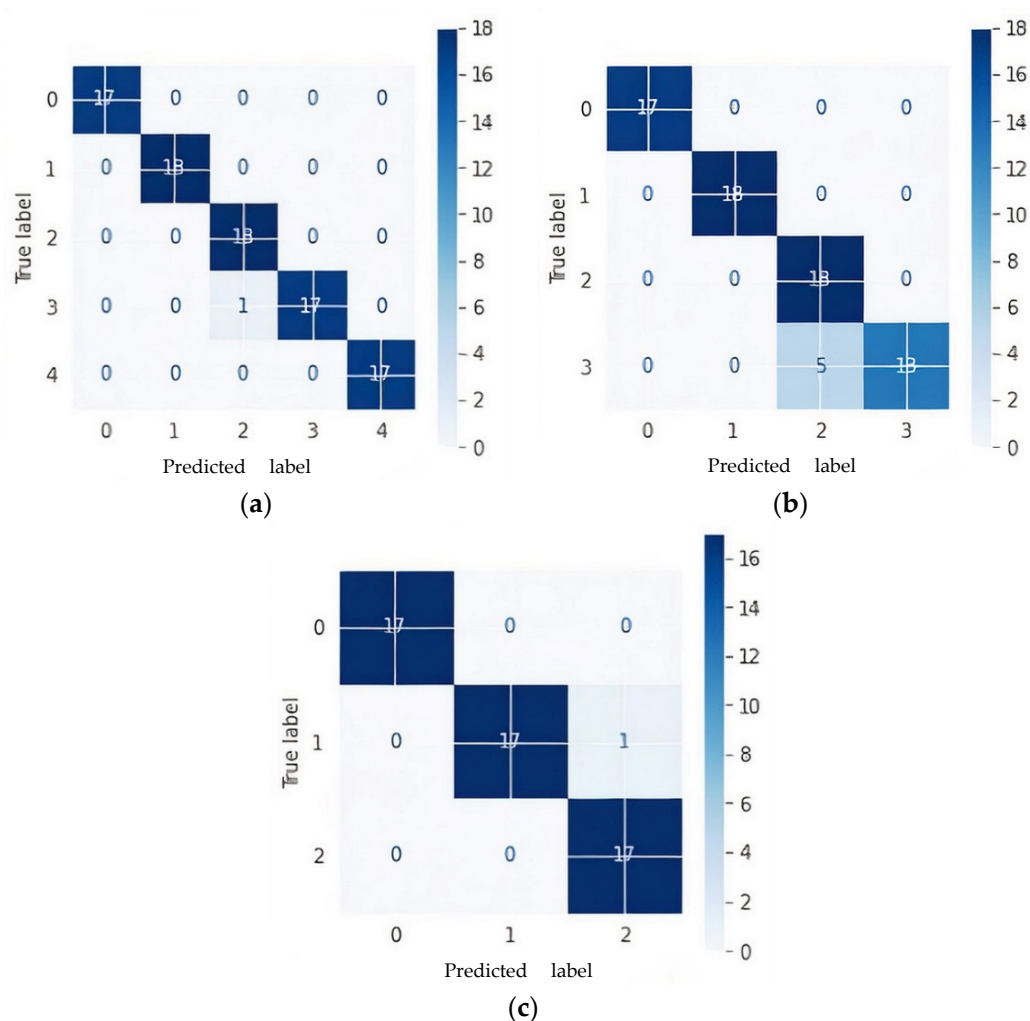
Figure 7. Confusion matrices of proposed model based on Kaiming weight initialization on test data: (a) 5-way multiclass; (b) 4-way multiclass; (c) 3-way multiclass.
