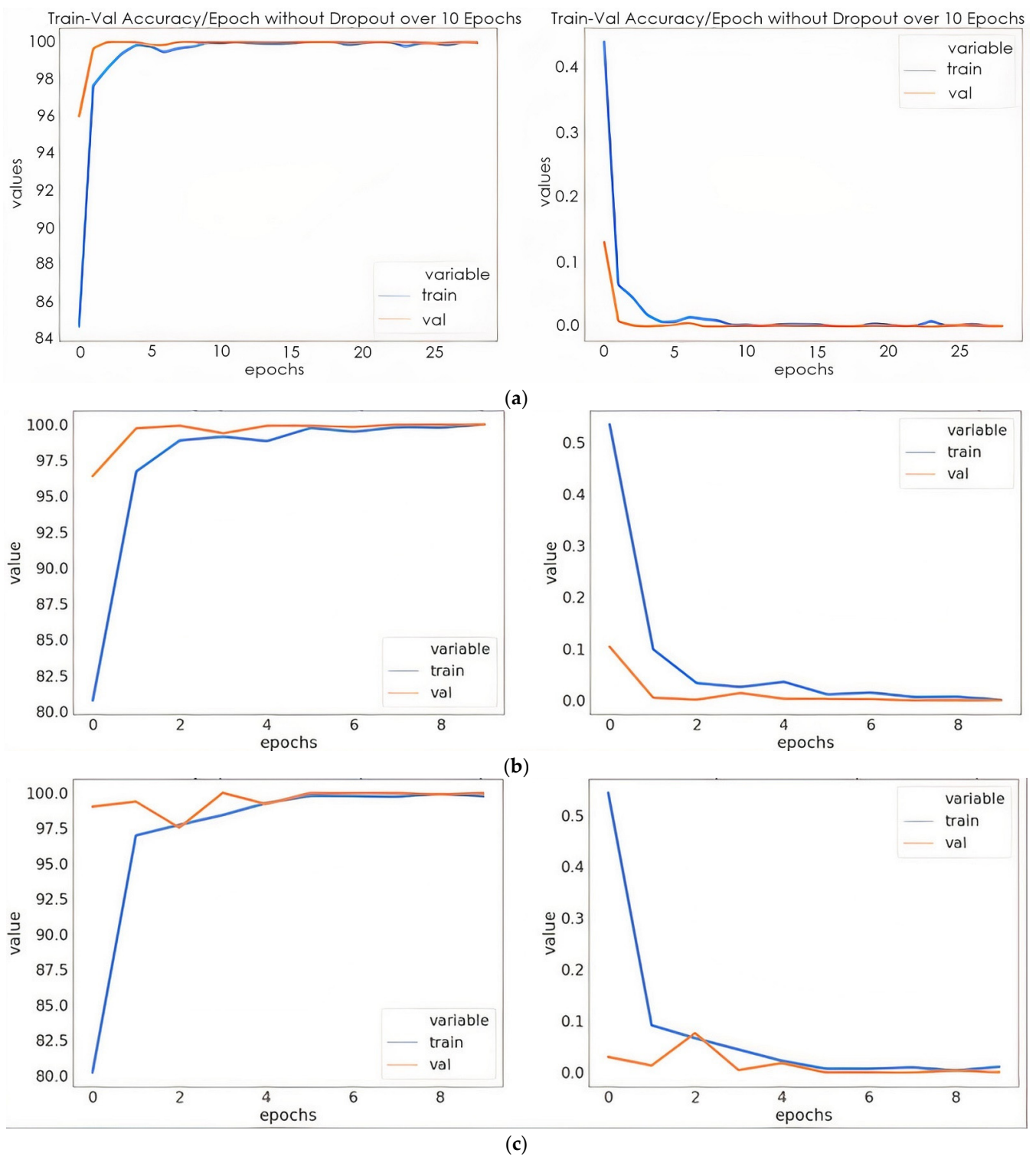
Figure 6. Training/validation accuracies and training loss/validation loss: (a) model without dropout; (b) mode with dropout; (c) model with dropout and weight decay discussions.
