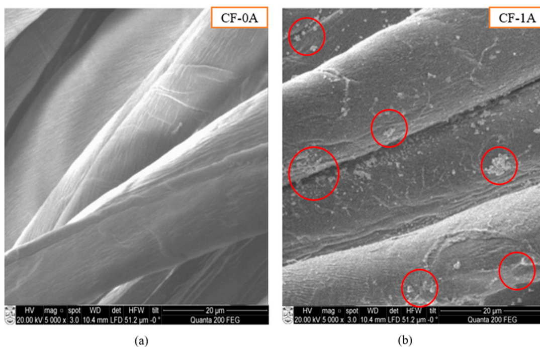
Figure 3. SEM images of the dyed cotton fabric: (a) without deposition of AgNPs (CF-0A); and (b) with deposition of AgNPs (CF-1A).
