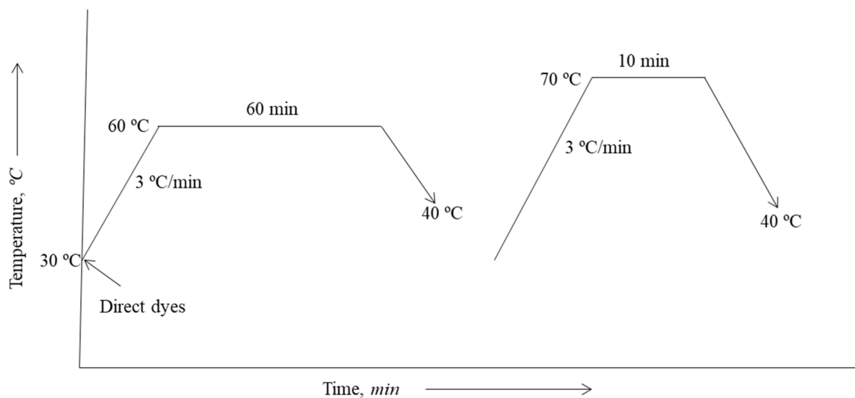
Figure 2. Process curve of direct dyeing.
