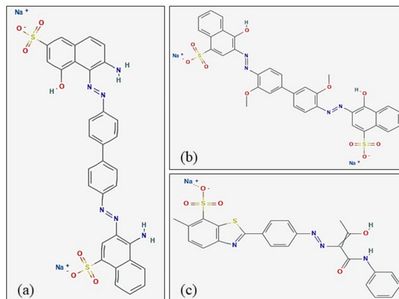
Figure 1. Chemical structure depiction of (a) C.I. Direct Red 13, (b) C.I. Direct Blue 8, and (c) C.I. Direct Yellow 8.
