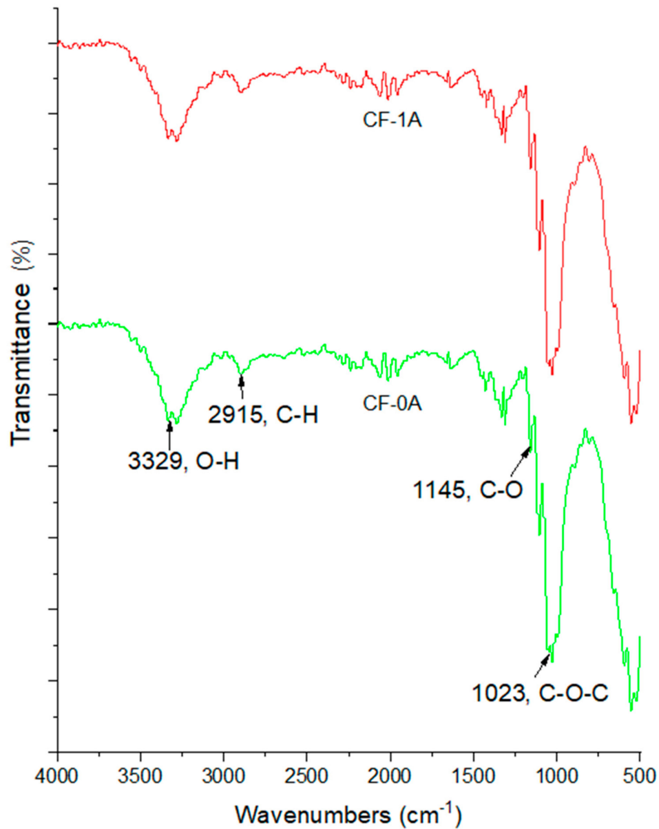
Figure 4. ATR-FTIR spectra of samples with and without deposition of AgNPs on the fabric surface.
