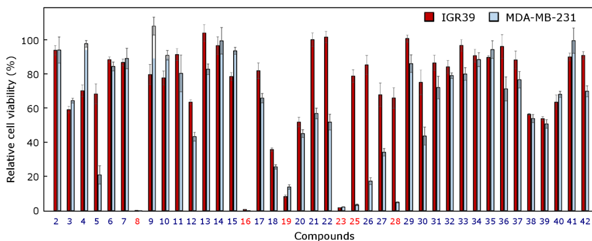
Figure 2. Effect of tested compounds on cancer cell viability at 100 µM concentration after 72 h of incubation, n = 3 . Experiments were repeated three times, calculating the mean and standard deviation. The number of the most active compounds selected for further experiments are shown in red.
