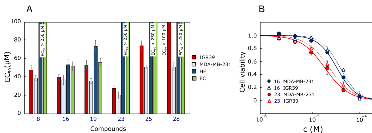
Figure 3. Effect of the most active compounds on cancer cell viability. (A). EC_{50} values of the most active compounds after 72 h of incubation by MTT assay. (B). Dose–response curves of compounds 16 and 23. n = 3 . Experiments were repeated three times, calculating the mean and standard deviation.
