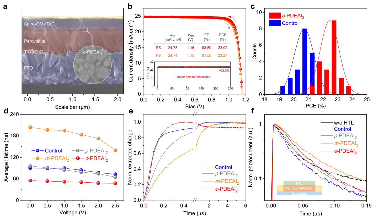
Fig. 3 Passivation layer-dependent device performance. a The cross-sectional scanning electron microscope (SEM) image of the PSC passivated with o -PDEAl 2 . b J - V characteristics of the champion device with o -PDEAl 2 measured in both reverse (red) and forward (orange) scanning directions (the inset shows its stabilized power output). c The statistics of PCE distribution for devices with and without o -PDEAl 2 . (Statistics from 20 samples for each condition). The solid lines denote the Gauss distribution fitting for the PCE statistics. d Voltage-dependent average PL lifetimes of the different devices. e Integrated charge extraction curves of devices. f Transient photocurrent decay in lateral sample geometry.
