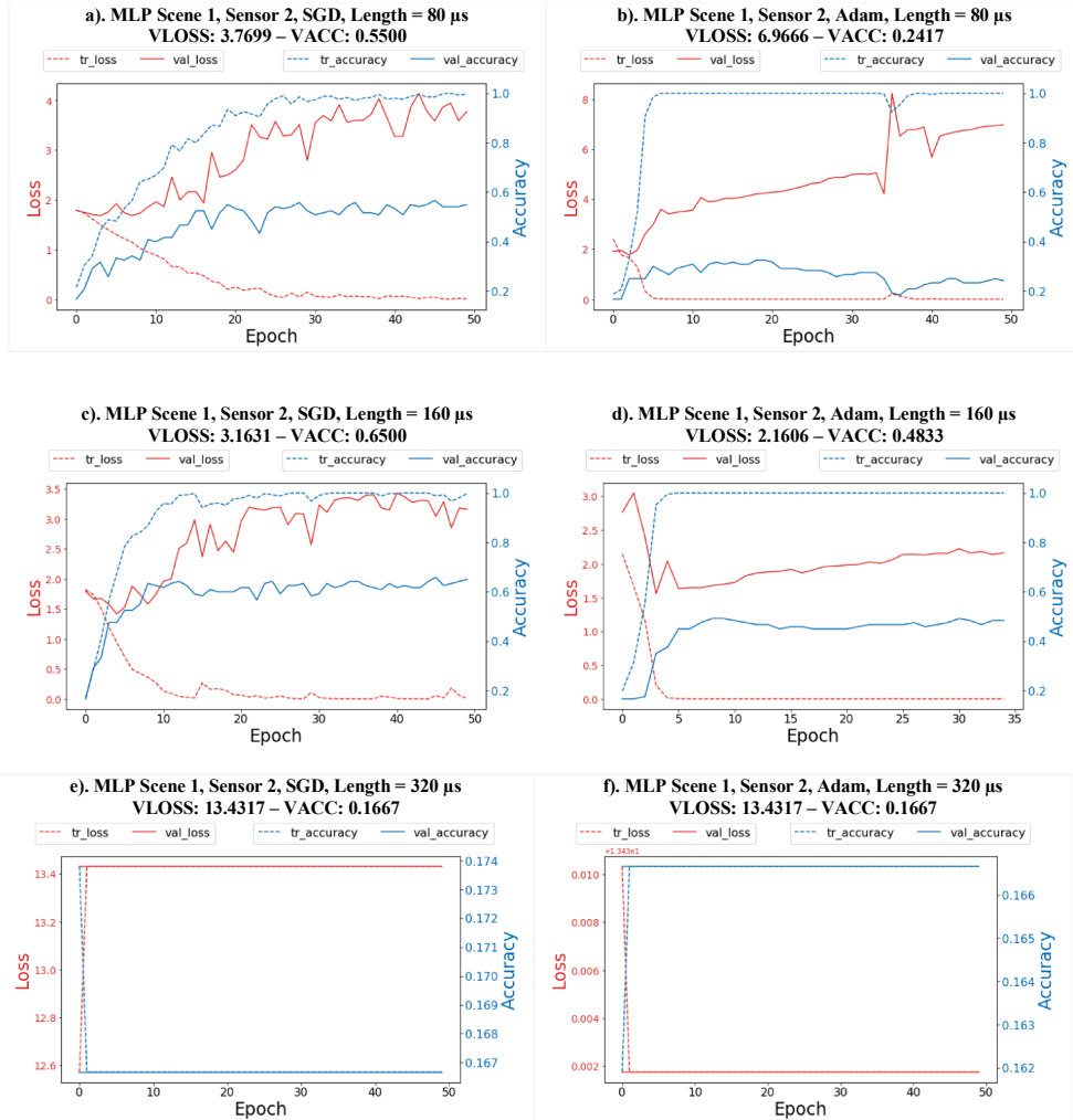
Fig. 17. a–f: Training results of MLP for signal from sensor 2 with various window length trained under Adam and SGD optimizer up to 50 epochs. 1 \mu\text{s} input length corresponds to 10 input samples. VACC = Final validation accuracy, VLOSS = Final Validation Loss. Note that the scaling is not uniform due to the default library settings.
