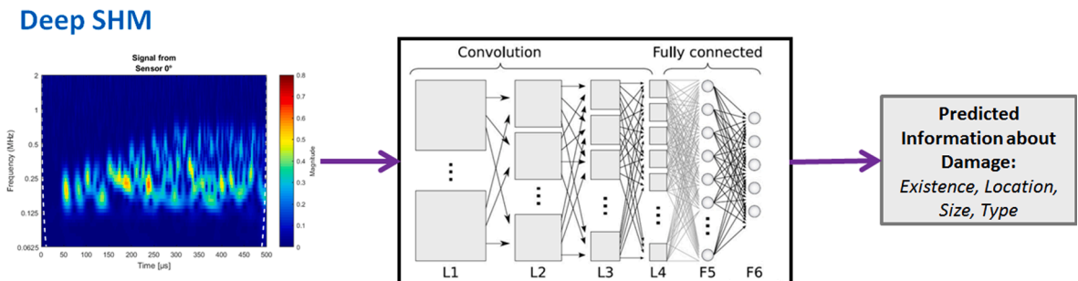
Fig. 4. DeepSHM Framework.
