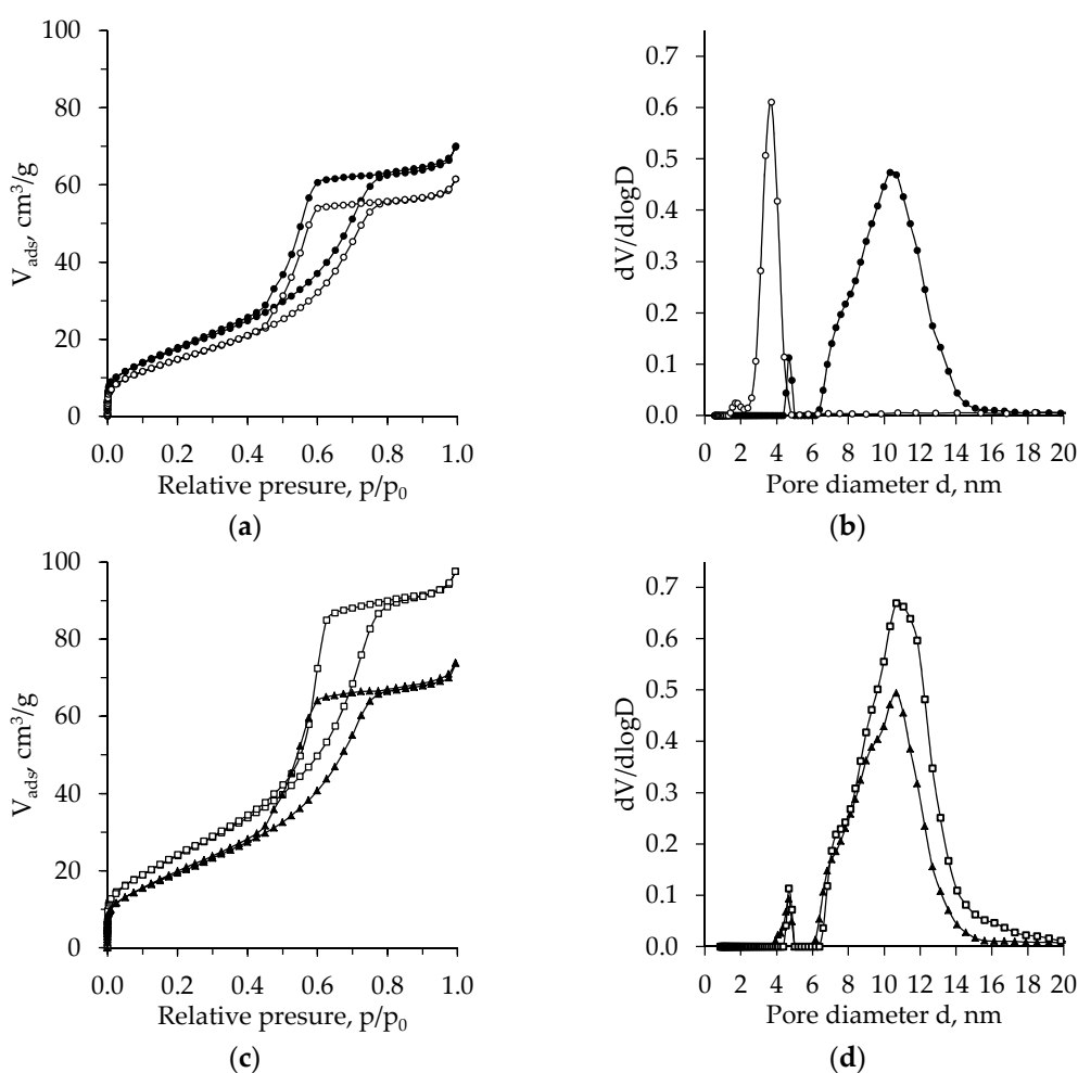
Figure 9. The BET adsorption–desorption isotherms (a,c) and pore size distribution (b,d) of calcinated TiO_2 aerogel vs. precursor (TBOT (a,b), TIP (c,d) and aging (●, ▲—unaged, ○, □—aged).
