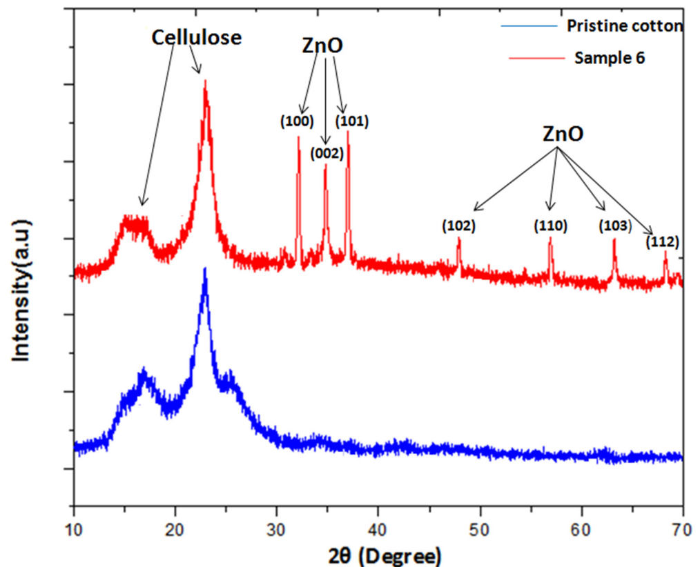
Figure 4. XRD diffractogram of pristine cotton and sample (6).
