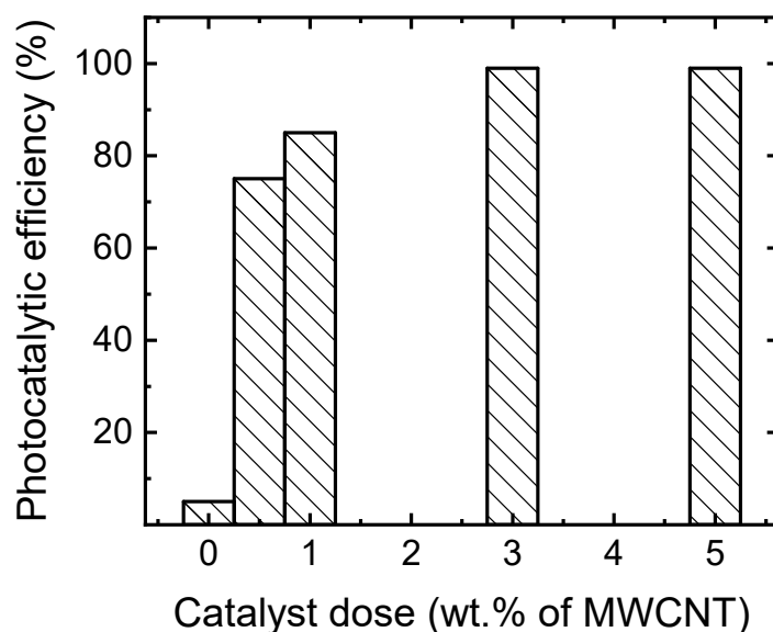
Figure 3. Effect of catalyst dose on the photocatalytic efficiency of Cr(VI) using the MWCNTs-Fe 3 O 4 @PES CNM.
